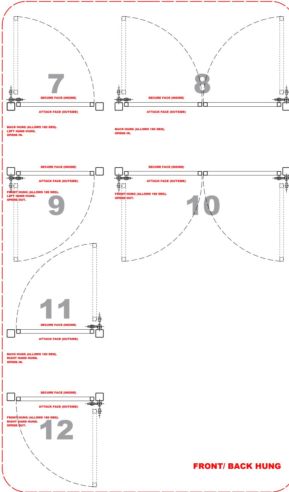
INLINE HUNG
